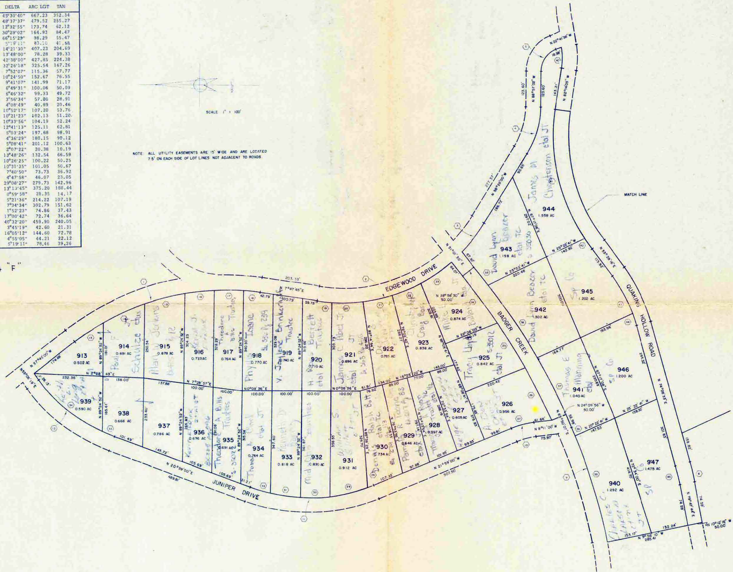
ASPEN HILLS SUBDIVISION CURVE TABLE
